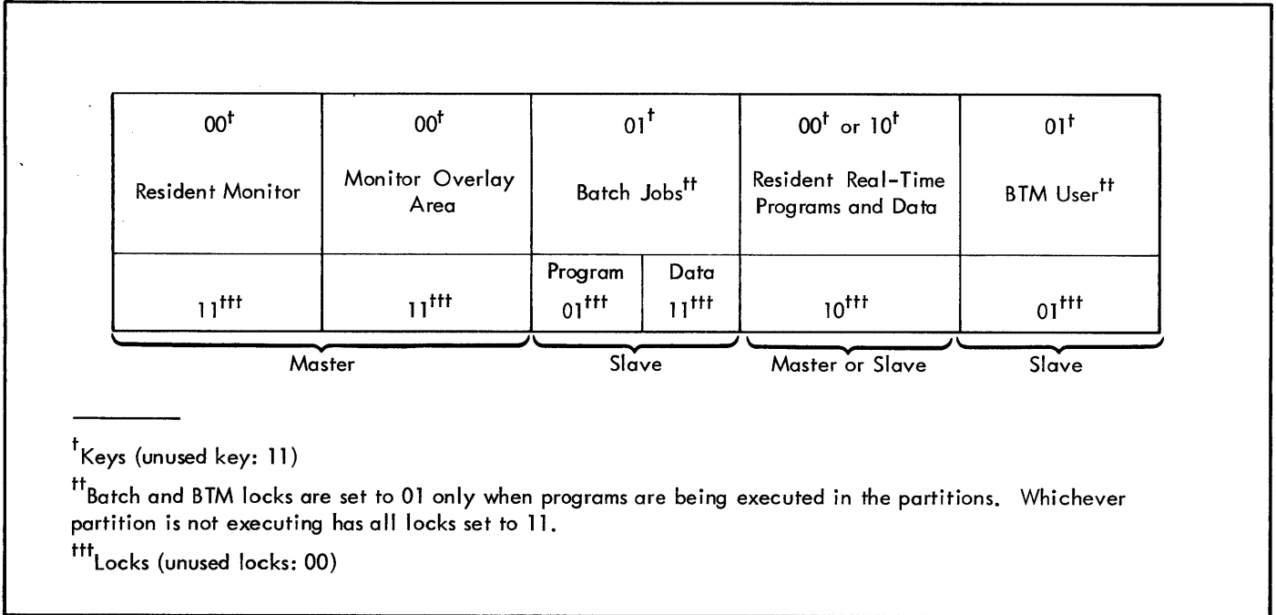
Figure 2. Typical Memory Layout (not to scale)
