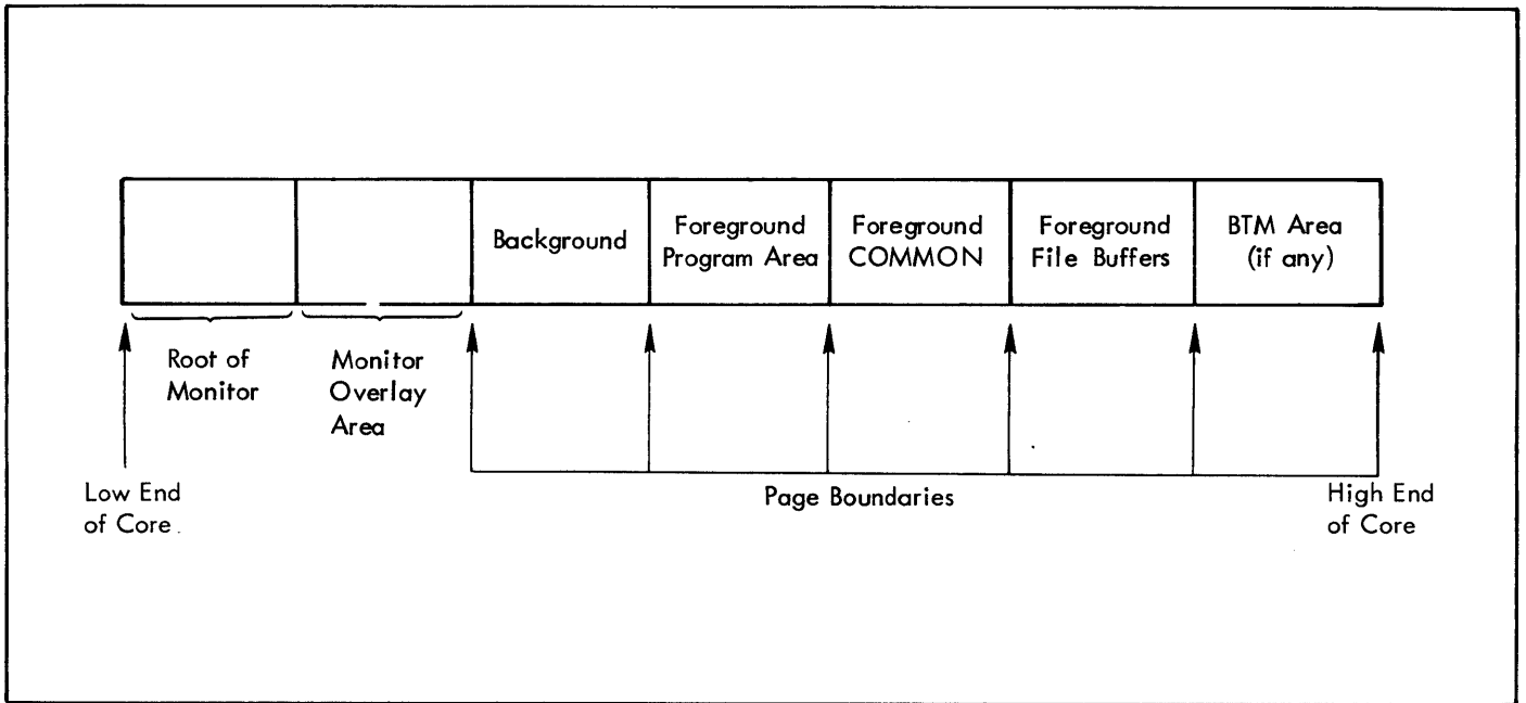
Figure 42. Real-Time System Memory Layout
