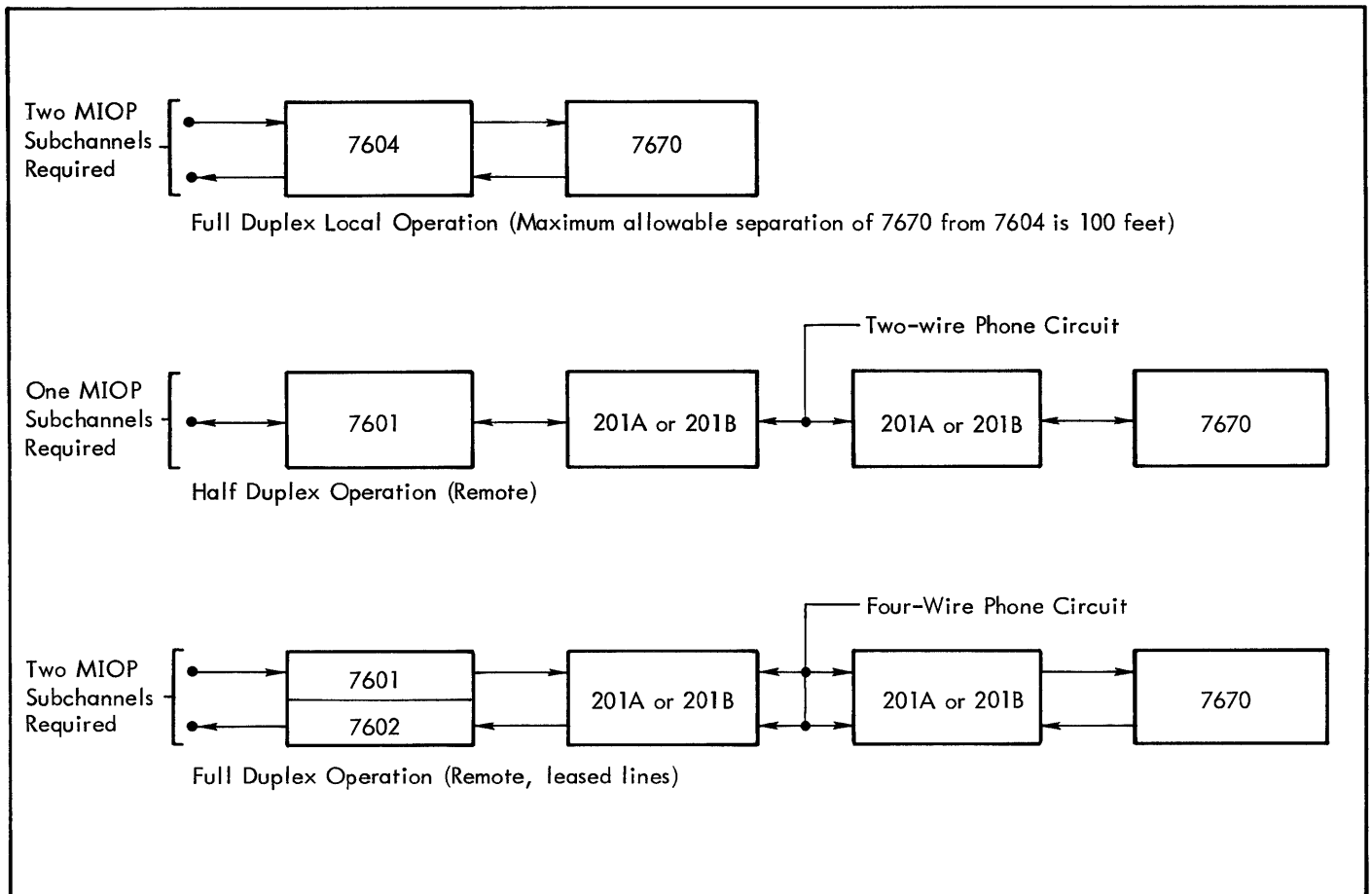
Figure 28. Remote Batch Terminal Hardware Configurations
