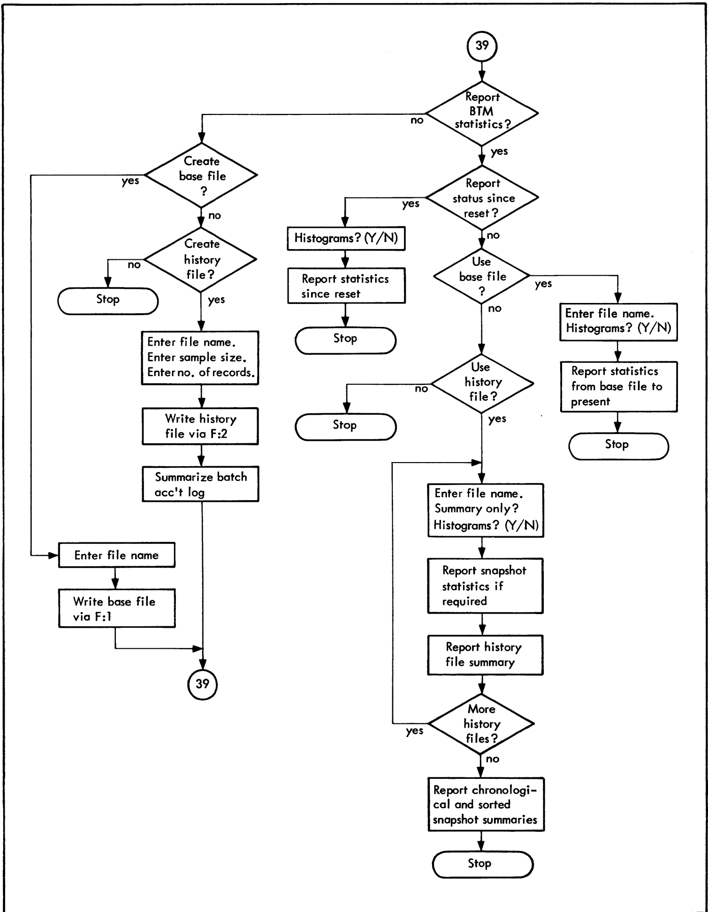
Figure 10. BTMPM Report Generator Flow Chart
