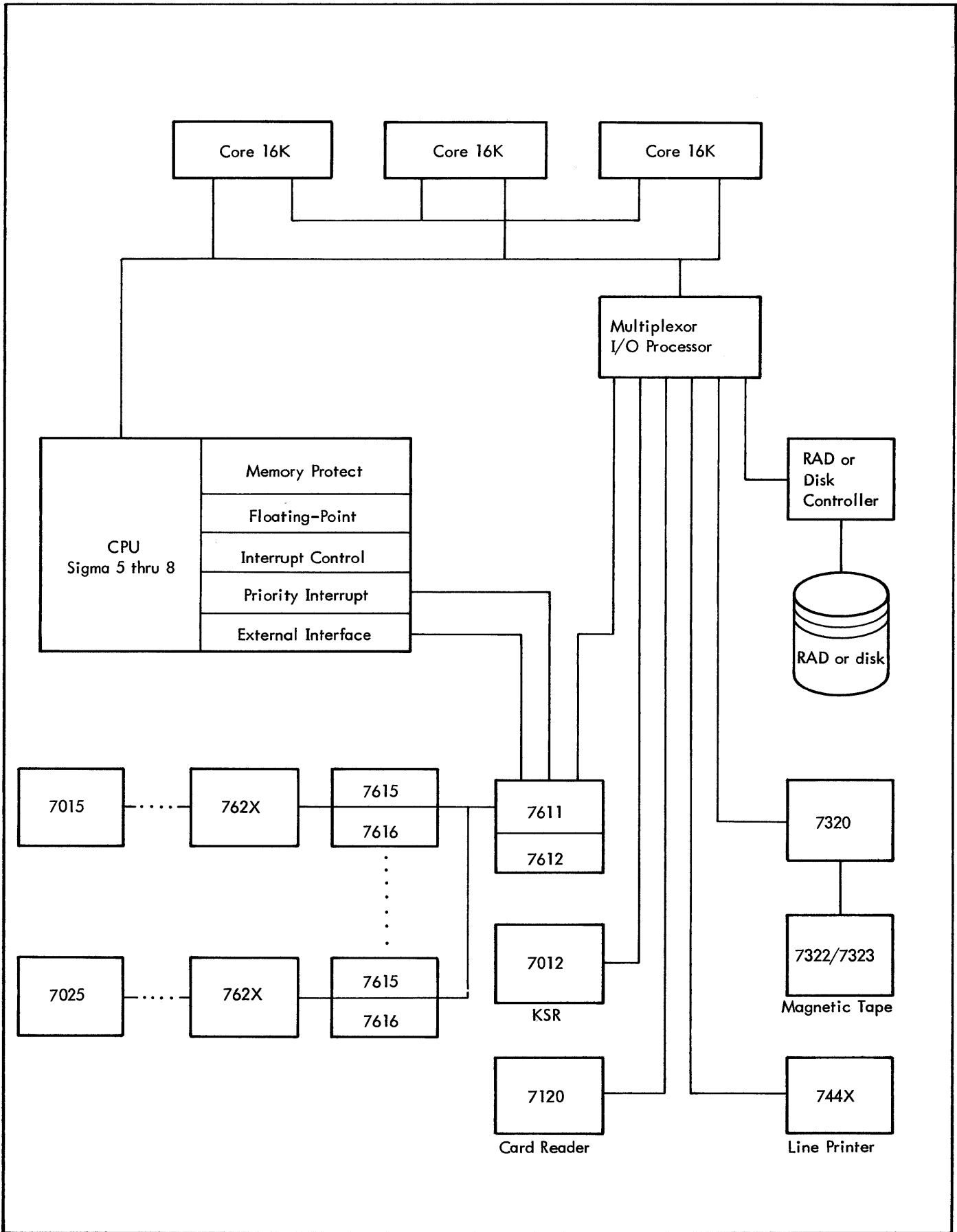
Figure 27. Typical BTM Hardware Configuration
