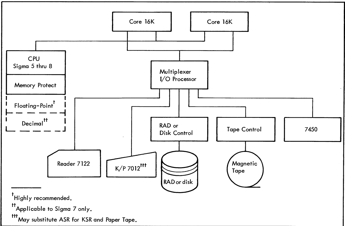
Figure 26. Sigma 5-8 Minimal BPM System
